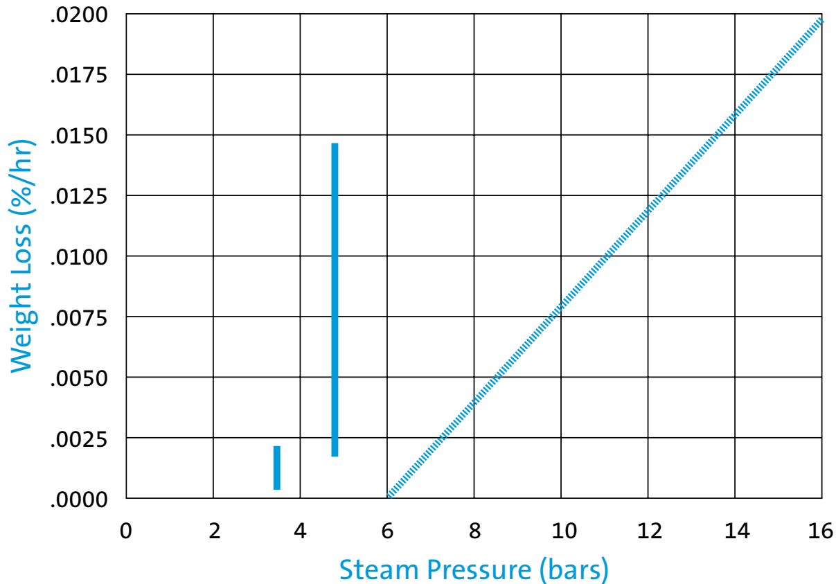
Comparison of BP Sunbury Results for Corrosion of Sintered Alpha SiC at 850°C vs. ORNL Results at 1177°C
