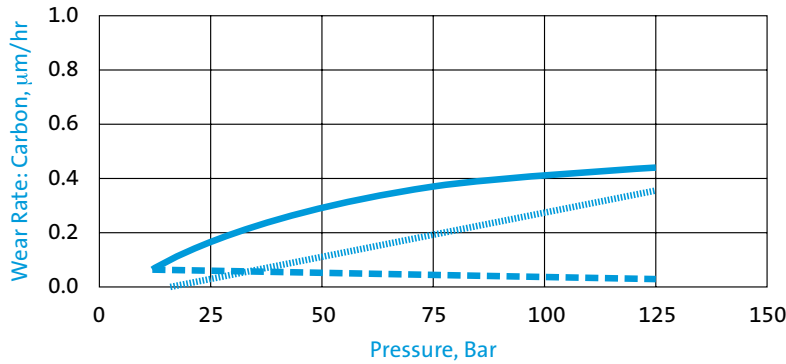
Wear Rate: SiC Primary Ring
